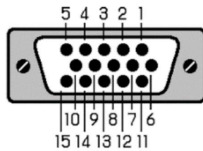
D-Sub female 15 pol:
